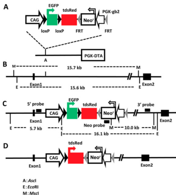
Fig.1 Generation of the ROSA26 locus with insertion of a novel Cre reporter.
